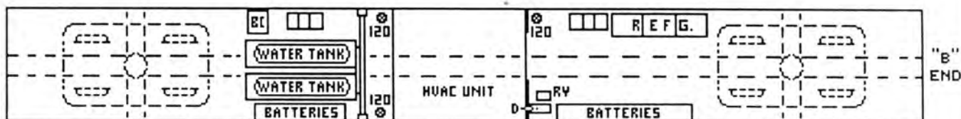
UNDERBODY VIEW THROUGH FLOOR
