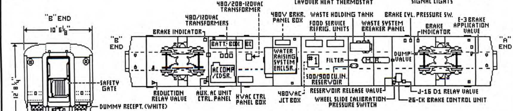
UNDERBODY VIEW THROUGH FLOOR
