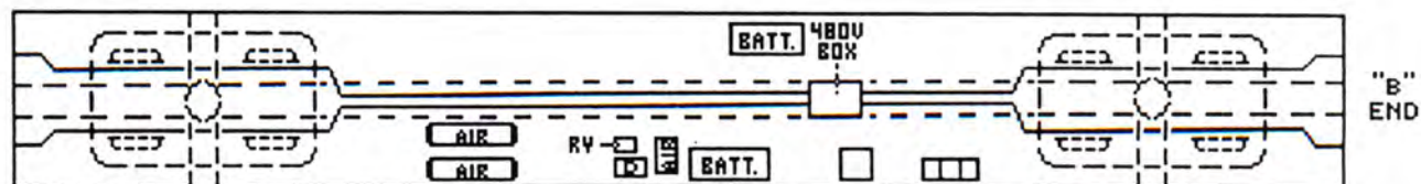
UNDERBODY VIEW THROUGH FLOOR
