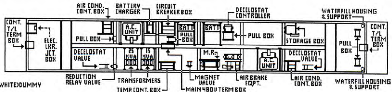
UNDERBODY VIEW THROUGH FLOOR
