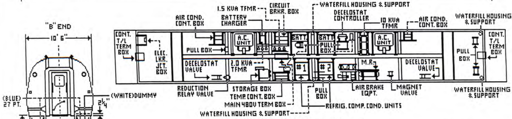
UNDERBODY VIEW THROUGH FLOOR * INCLUDES A.D.A. MODIFICATIONS *
