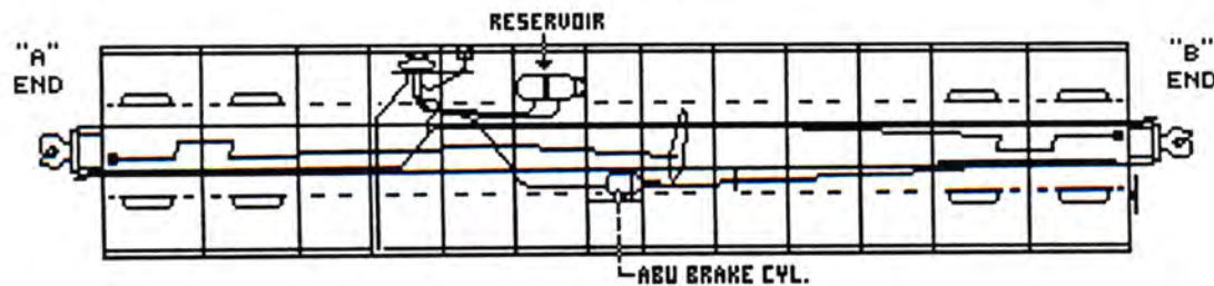
UNDERBODY VIEW THROUGH FLOOR
