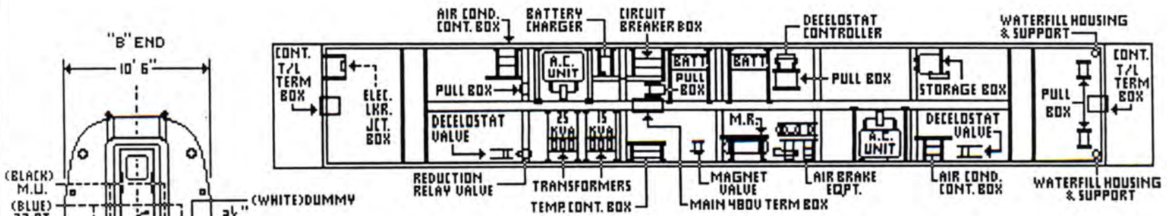
UNDERBODY VIEW THROUGH FLOOR
