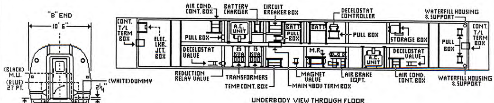
UNDERBODY VIEW THROUGH FLOOR
