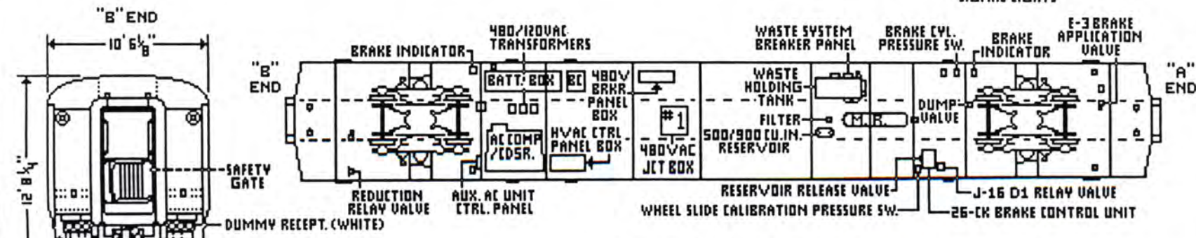
UNDERBODY VIEW THROUGH FLOOR
