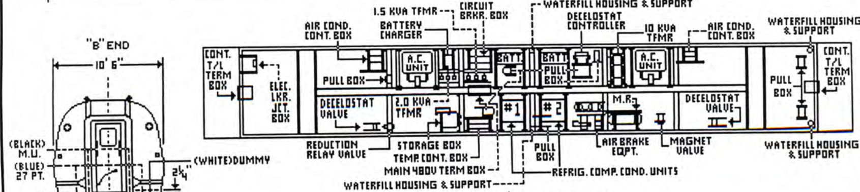
UNDERBODY VIEW THROUGH FLOOR * INCLUDES A.D.A. MODIFICATIONS *
