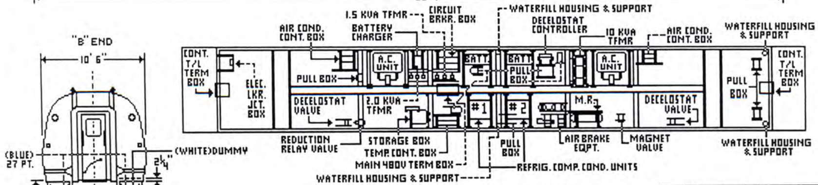
UNDERBODY VIEW THROUGH FLOOR
