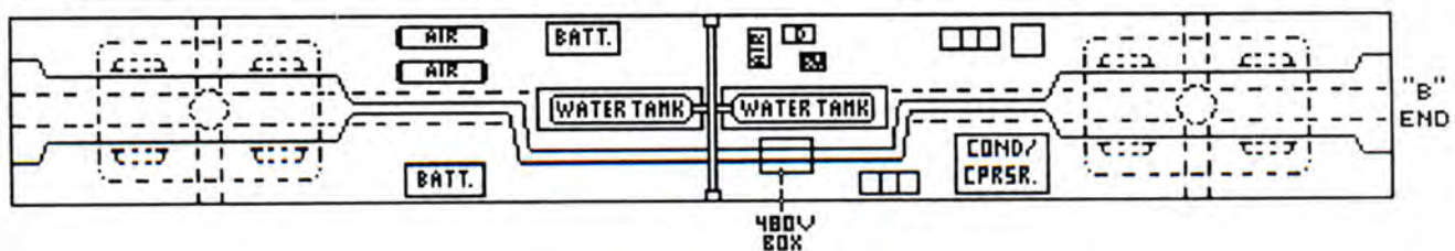
UNDERBODY VIEW THROUGH FLOOR
